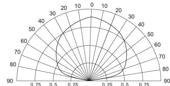
Candle Power Distribution Curve
